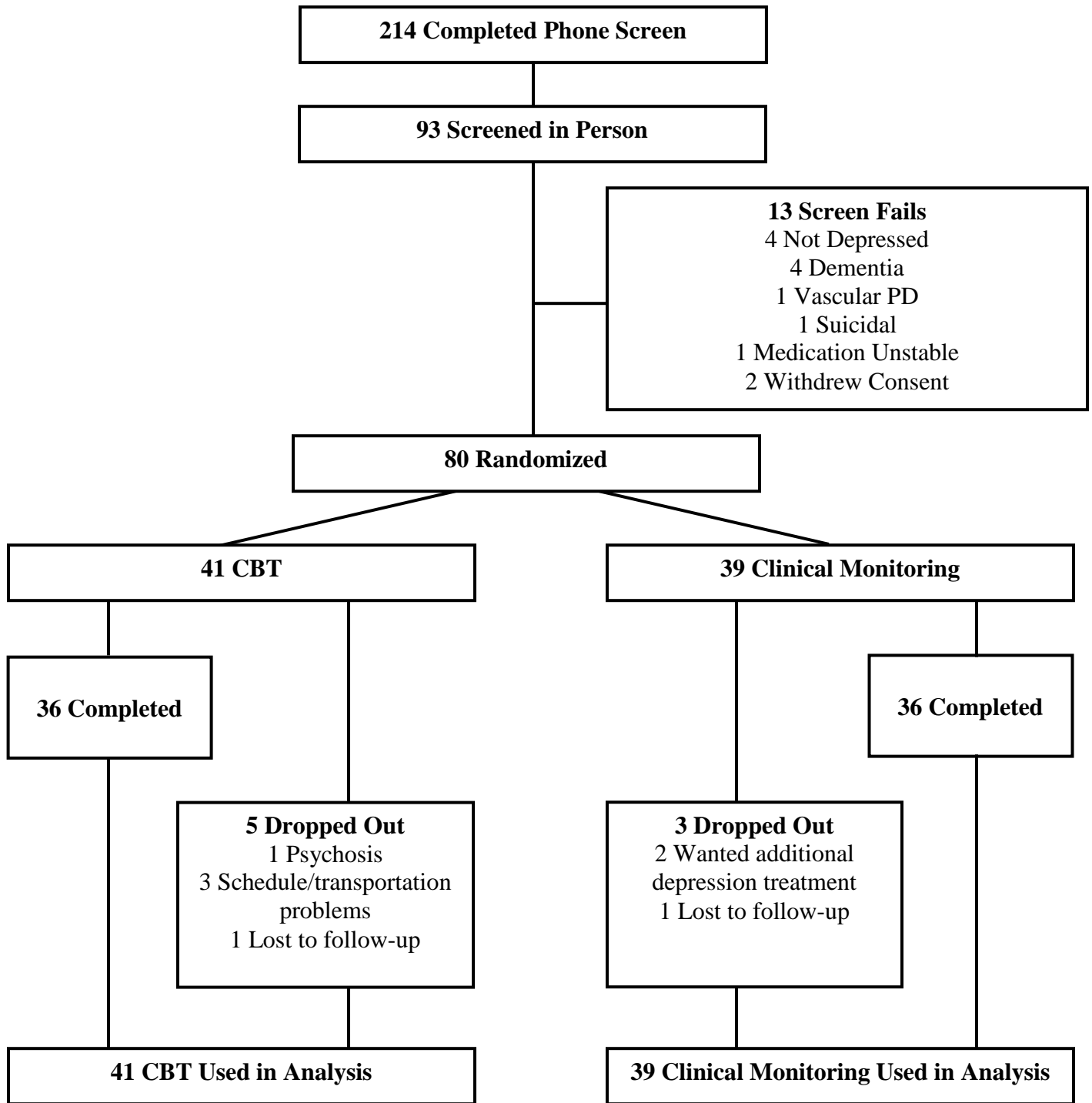
Figure 1. CONSORT Diagram
