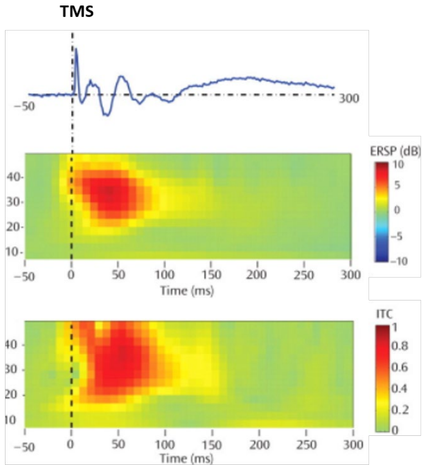
Supp. Fig 1. TMS-evoked EEG response (Top) with related ERSP (middle) and ITC (bottom) activity.
